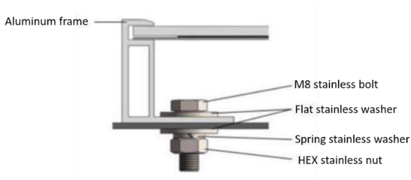
Figure 1. PV module installed with bolt fitting method.
